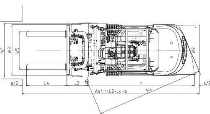
RASA: Right angle stacking aisle width
