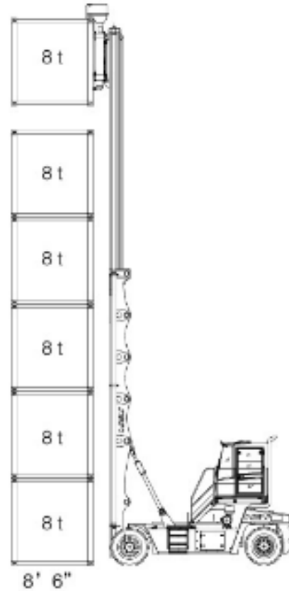
CPCD180EC6-CZ
